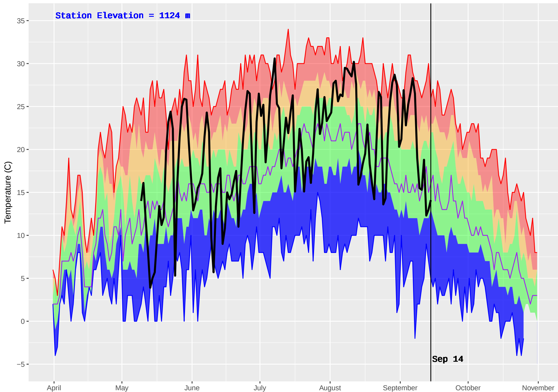
COLDSCAUR LAKE (232) : Historical (1979–2016) and Current (2017) Noon Temperature
